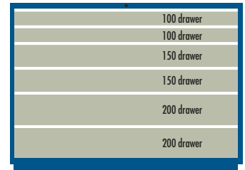
Total drawer height = 900
