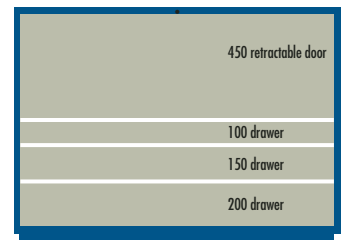
Total drawer and door height = 900
