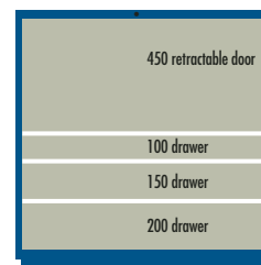
Total drawer and door height = 900
