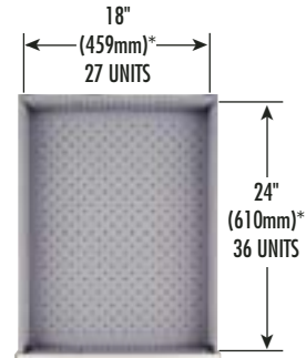
*inside dimensions
